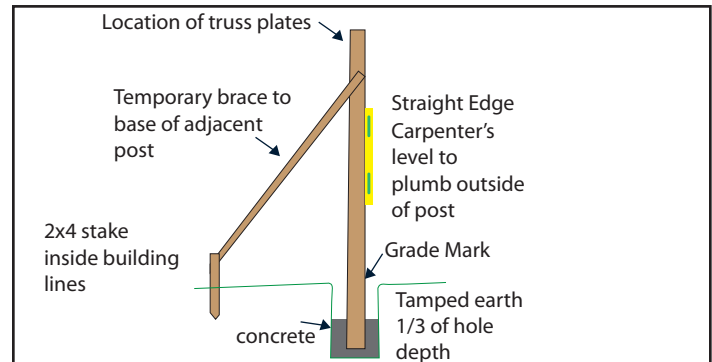
Figure 7. Alignment and temporary bracing of posts (Steps 11 and 12)
