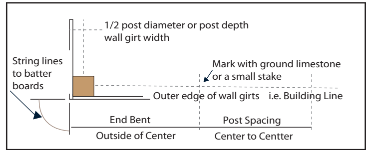
Figure 6. Location posts and string lines (Step 10)
